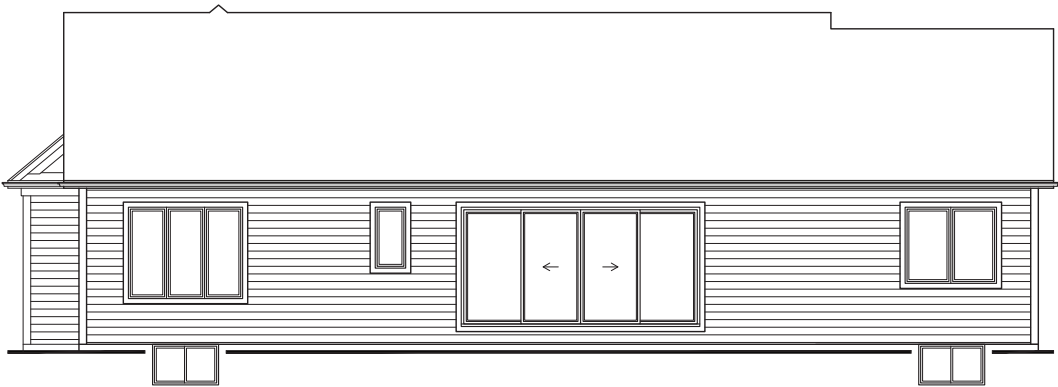
REAR ELEVATION
